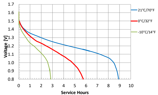
Constant Current - 100 mA
